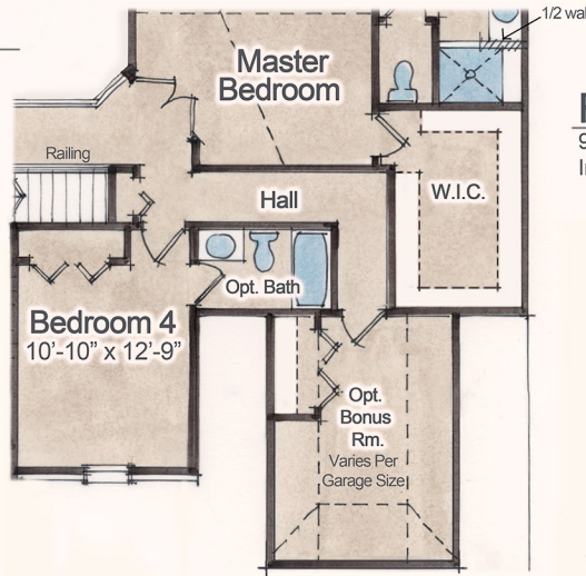
Opt. Bonus Room 2 Car or 3 Car Front Entry Only +305 S.F. With 3rd Bath & Larger W.I.C.
