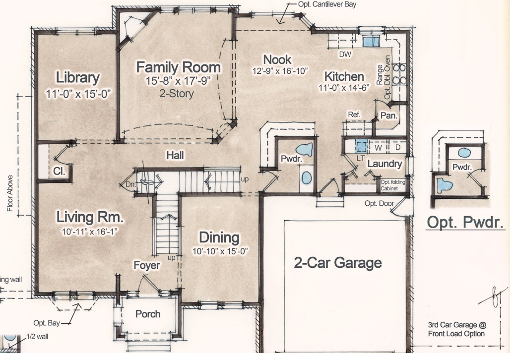
First Floor Plan 1,802 sq. ft. 9' Standard First Floor Ceilings. Interior Radius Archways Are Optional.
